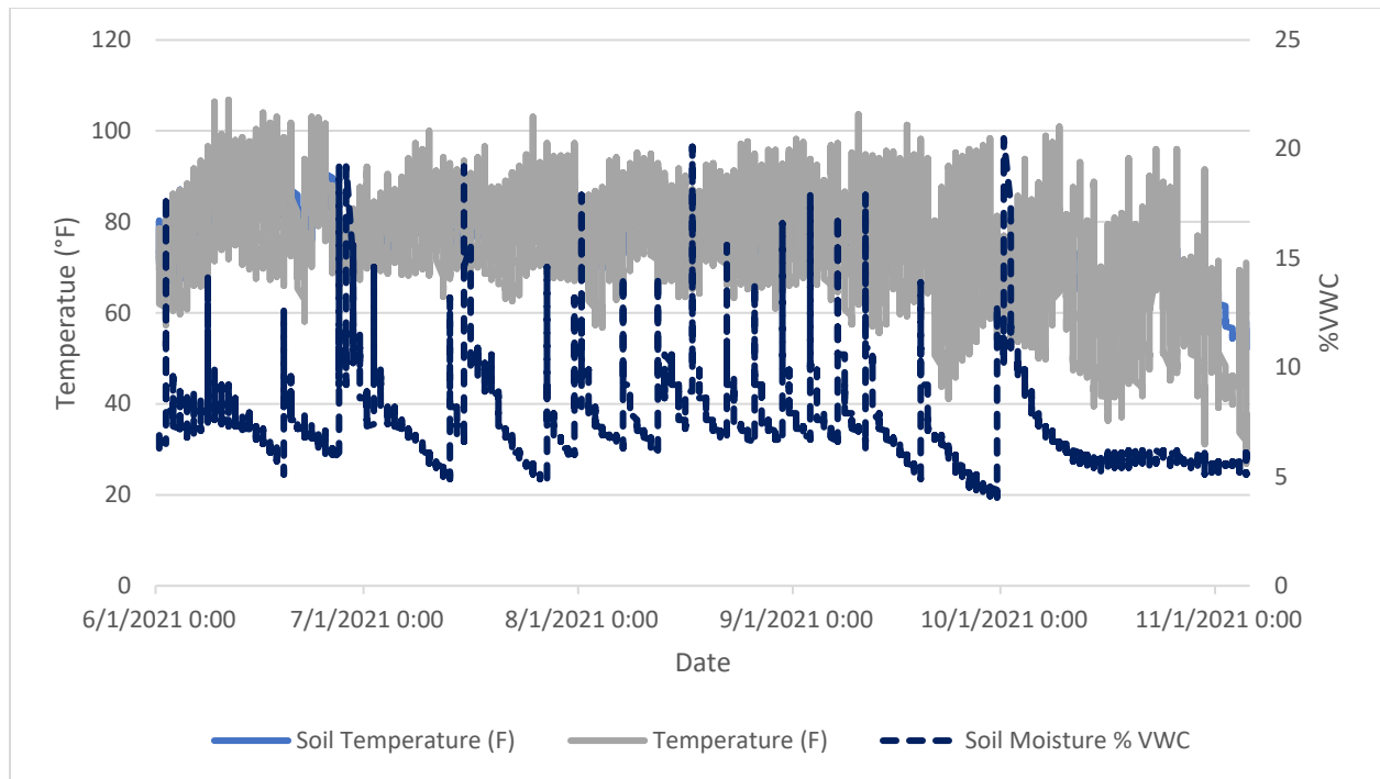
Figure 1: Soil temperature (°F), soil moisture (%VWC) and temperature (°F) from June 01 to November 05, 2021
